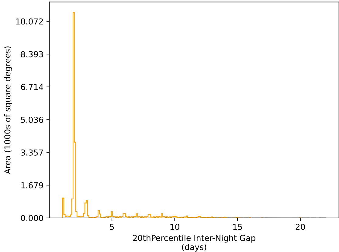
too_elab_r16_d3_ugrizy_v3.4_10yrs All sky r band: 20thPercentile Inter-Night Gap
