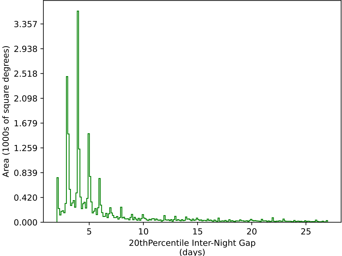
too_elab_r16_d3_ugrizy_v3.4_10yrs All sky g band: 20thPercentile Inter-Night Gap
