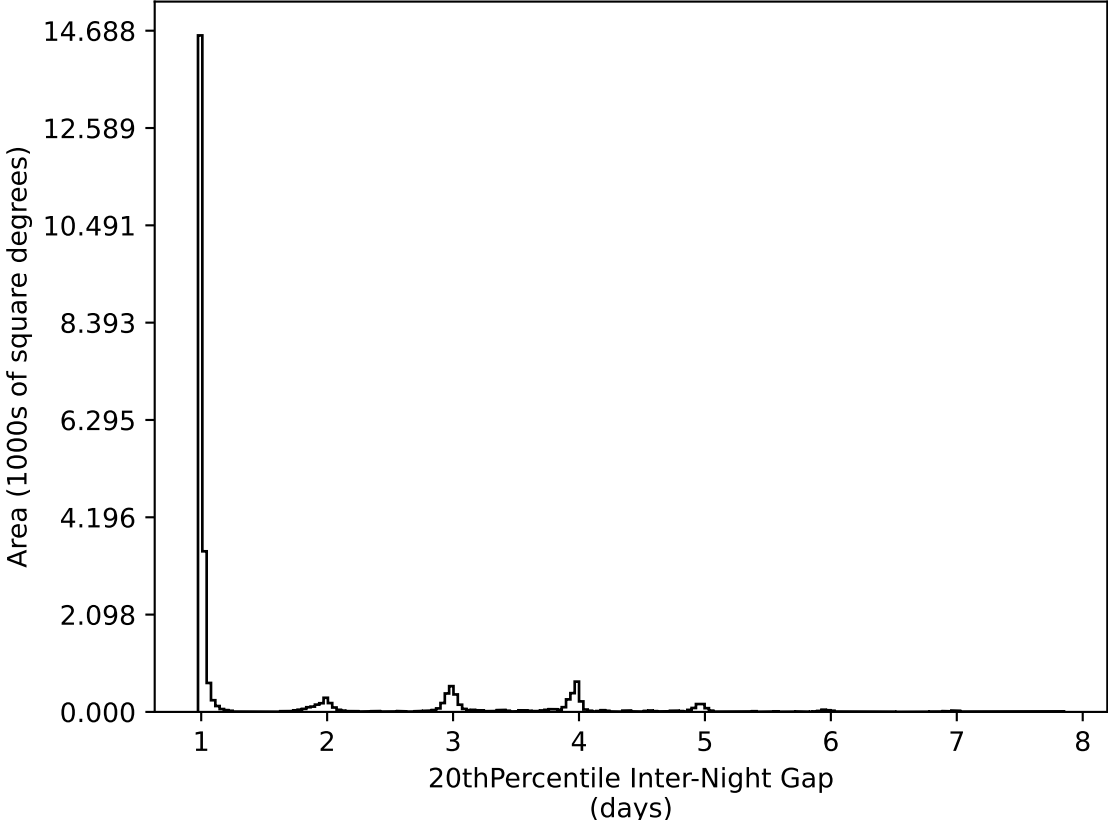
too_elab_r16_d3_ugrizy_v3.4_10yrs All sky all bands: 20thPercentile Inter-Night Gap
