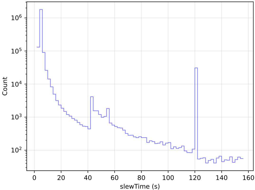
too_elab_r16_d3_ugrizy_v3.4_10yrs All visits: Slew Time Histogram
