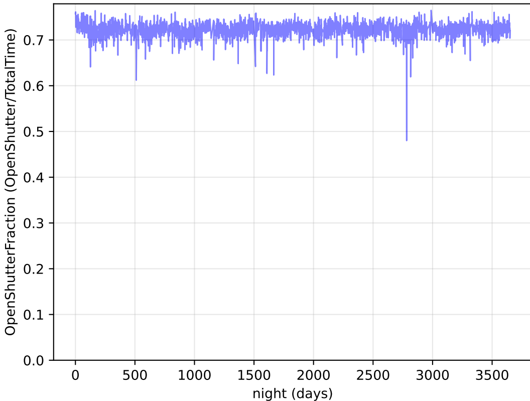
too_elab_r16_d3_ugrizy_v3.4_10yrs : OpenShutterFraction
