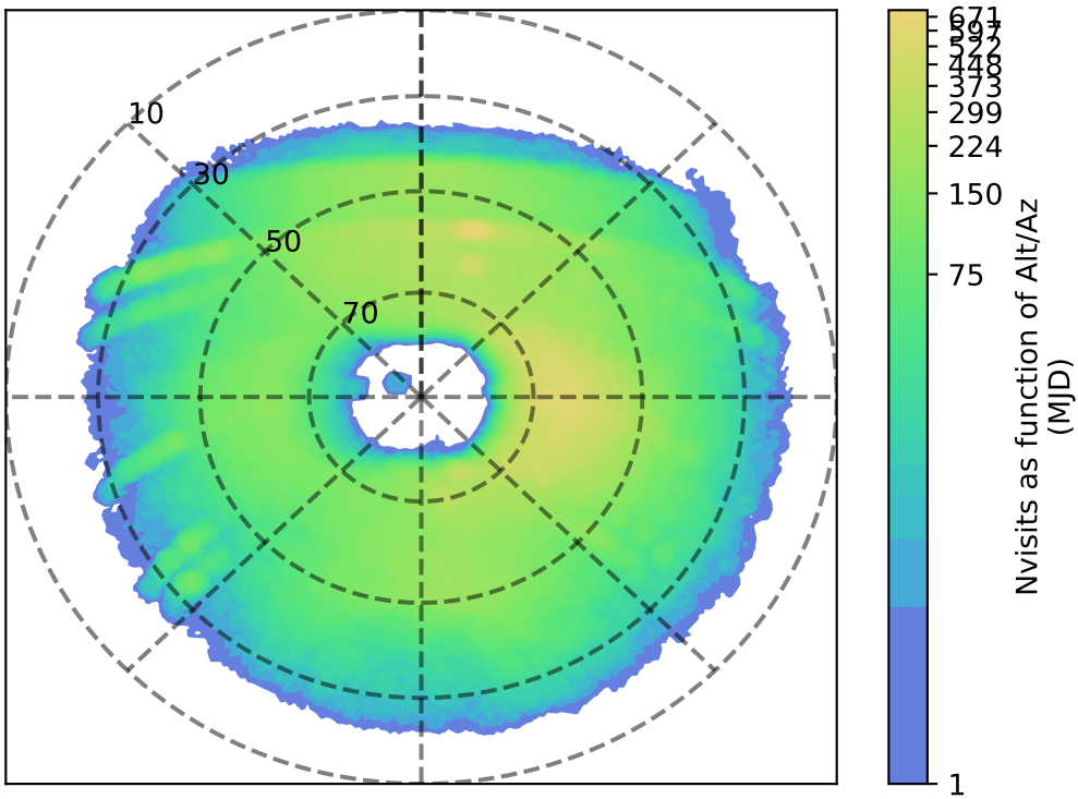
too_elab_r16_d3_ugrizy_v3.4_10yrs u: Nvisits as function of Alt/Az
