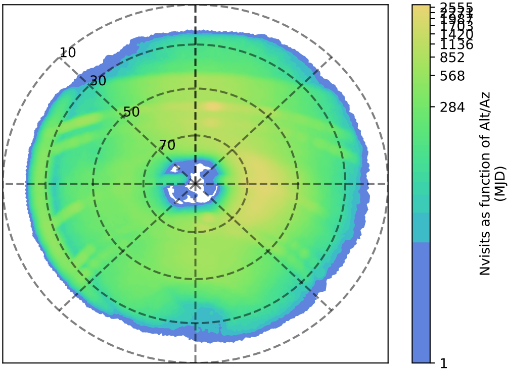
too_elab_r16_d3_ugrizy_v3.4_10yrs r: Nvisits as function of Alt/Az
