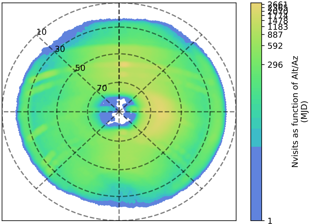
too_elab_r16_d3_ugrizy_v3.4_10yrs i: Nvisits as function of Alt/Az
