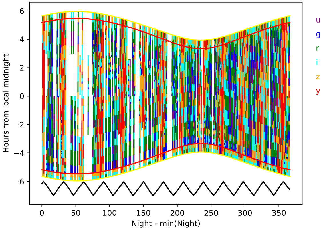
too_elab_r16_d3_ugrizy_v3.4_10yrs year 9-10: Hourglass
