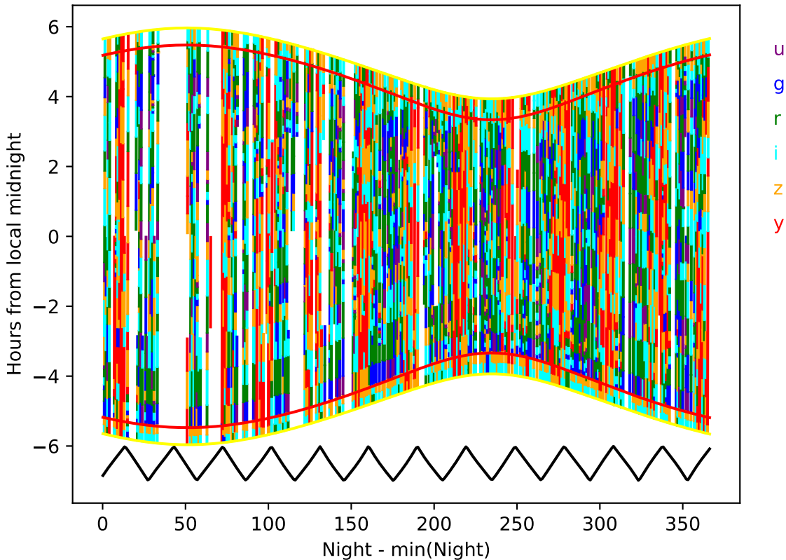
too_elab_r16_d3_ugrizy_v3.4_10yrs year 8-9: Hourglass
