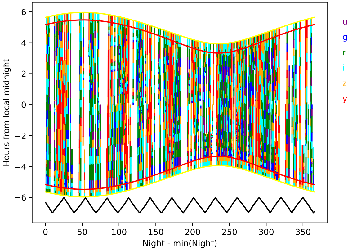
too_elab_r16_d3_ugrizy_v3.4_10yrs year 7-8: Hourglass
