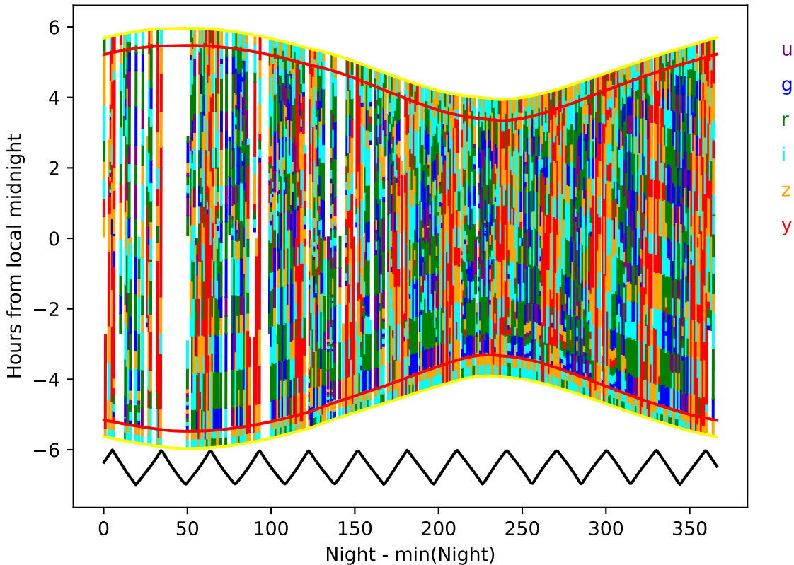
too_elab_r16_d3_ugrizy_v3.4_10yrs year 6-7: Hourglass
