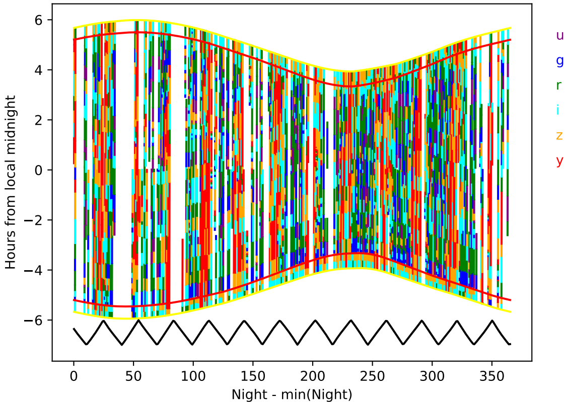
too_elab_r16_d3_ugrizy_v3.4_10yrs year 4-5: Hourglass
