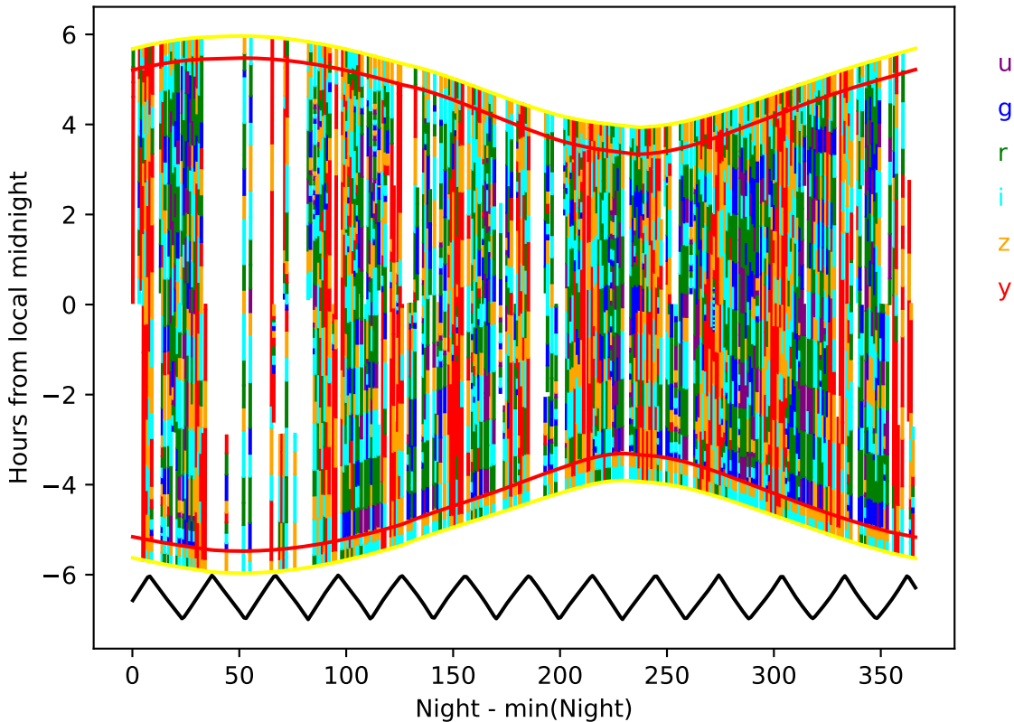
too_elab_r16_d3_ugrizy_v3.4_10yrs year 3-4: Hourglass
