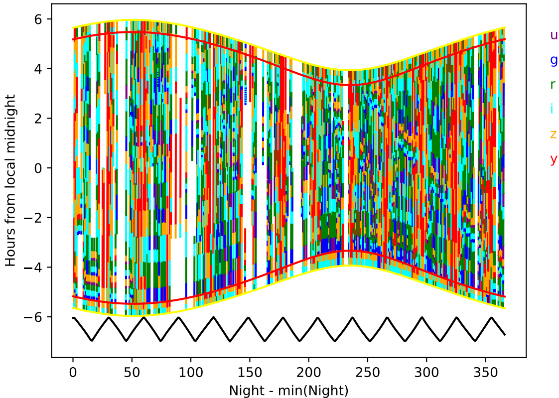
too_elab_r16_d3_ugrizy_v3.4_10yrs year 1-2: Hourglass
