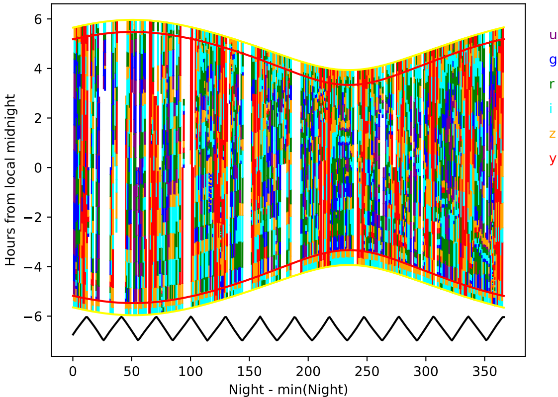
too_elab_r16_d3_ugrizy_v3.4_10yrs year 0-1: Hourglass
