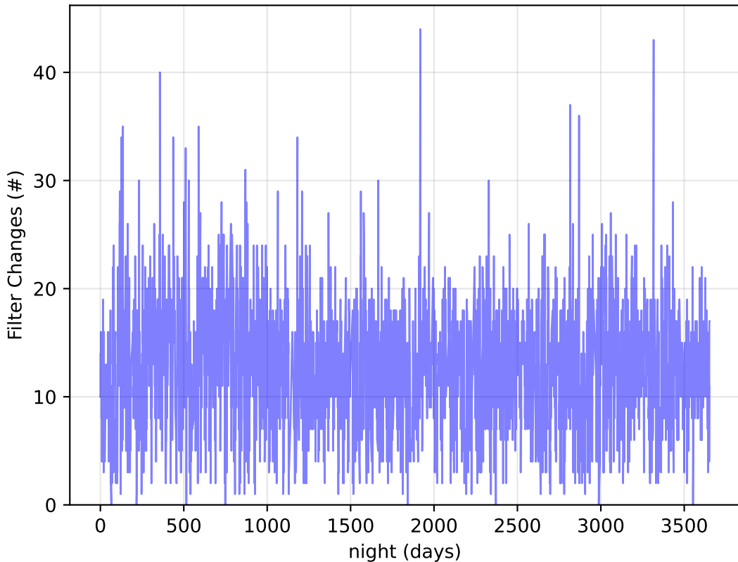
too_elab_r16_d3_ugrizy_v3.4_10yrs : Filter Changes
