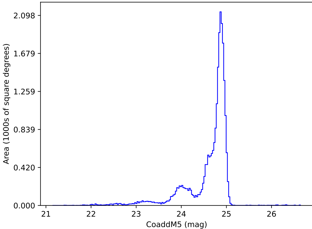
too_elab_r16_d3_ugrizy_v3.4_10yrs y: CoaddM5
