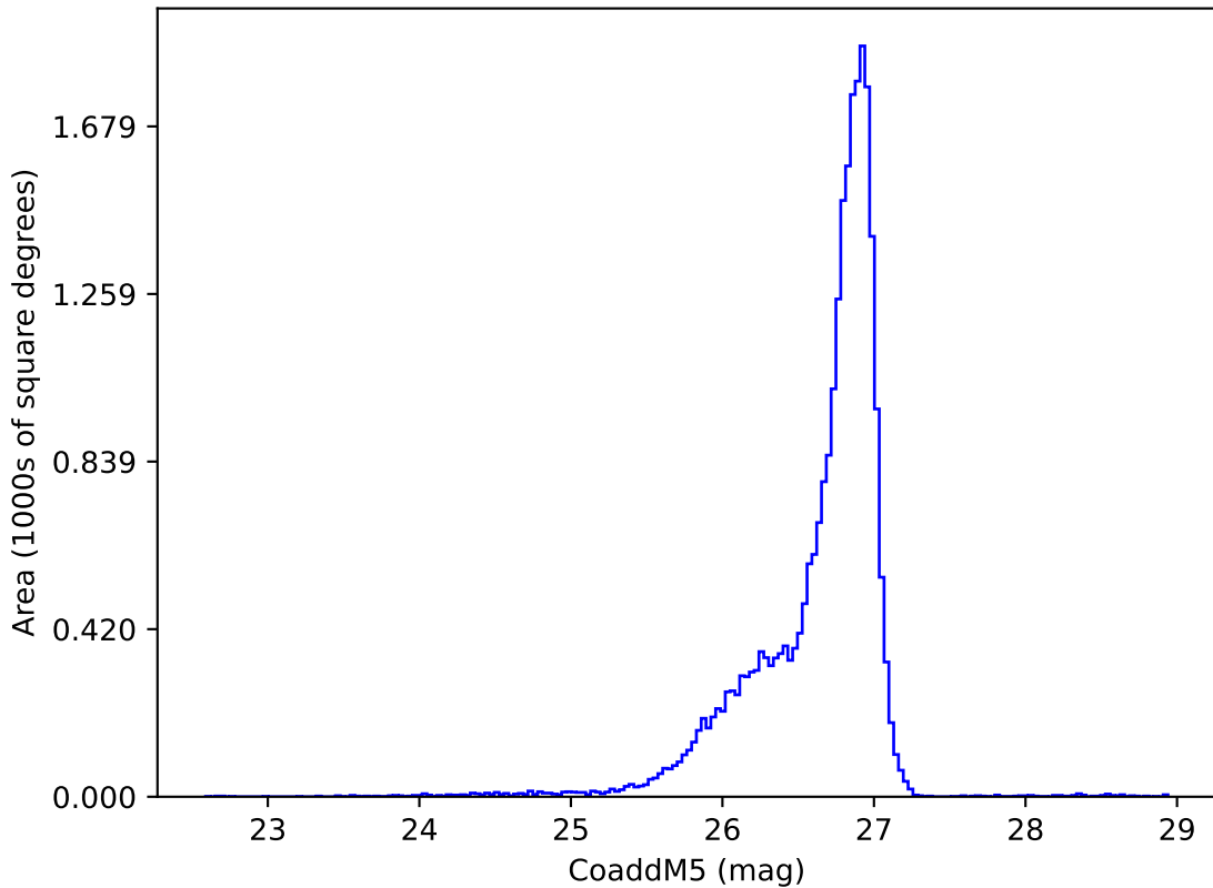
too_elab_r16_d3_ugrizy_v3.4_10yrs g: CoaddM5
