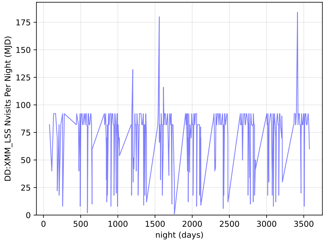
too_elab_r16_d3_ugrizy_v3.4_10yrs all bands: DD:XMM_LSS Nvisits Per Night
