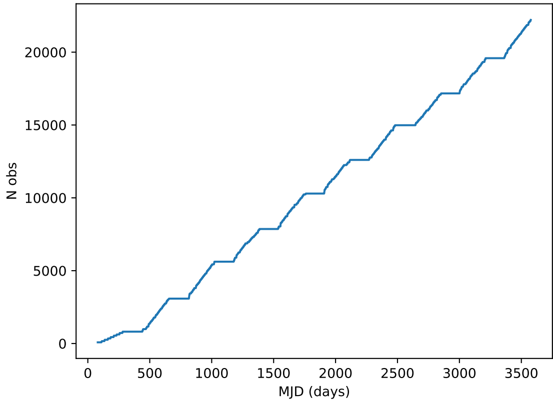
too_elab_r16_d3_ugrizy_v3.4_10yrs all bands: DD:XMM_LSS Cumulative NVisits
