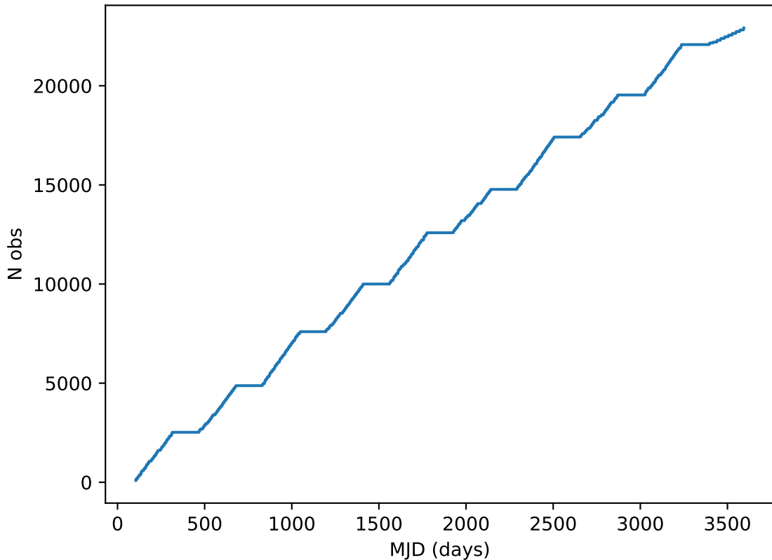
too_elab_r16_d3_ugrizy_v3.4_10yrs all bands: DD:EDFS Cumulative NVisits
