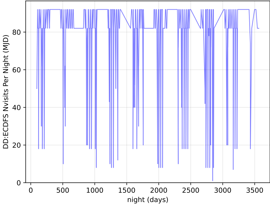
too_elab_r16_d3_ugrizy_v3.4_10yrs all bands: DD:ECDFS Nvisits Per Night
