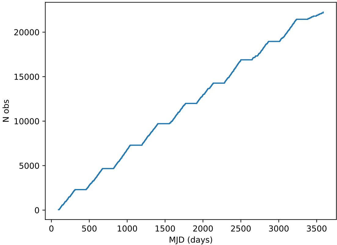
too_elab_r16_d3_ugrizy_v3.4_10yrs all bands: DD:ECDFS Cumulative NVisits
