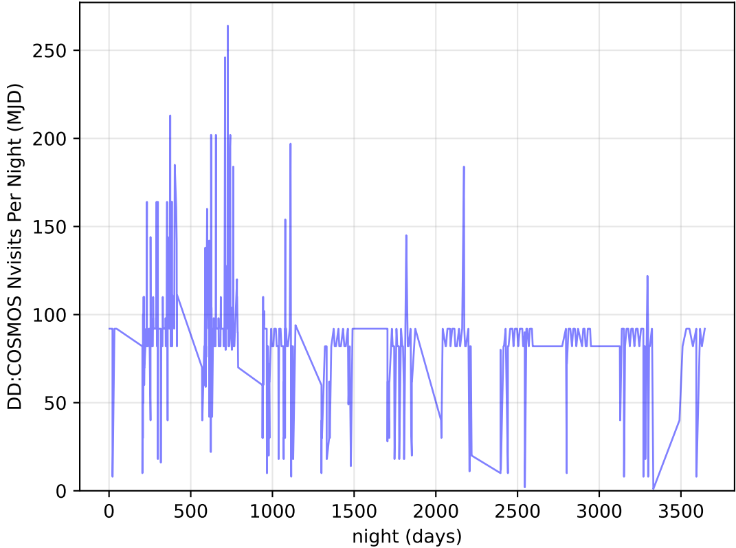
too_elab_r16_d3_ugrizy_v3.4_10yrs all bands: DD: COSMOS Nvisits Per Night
