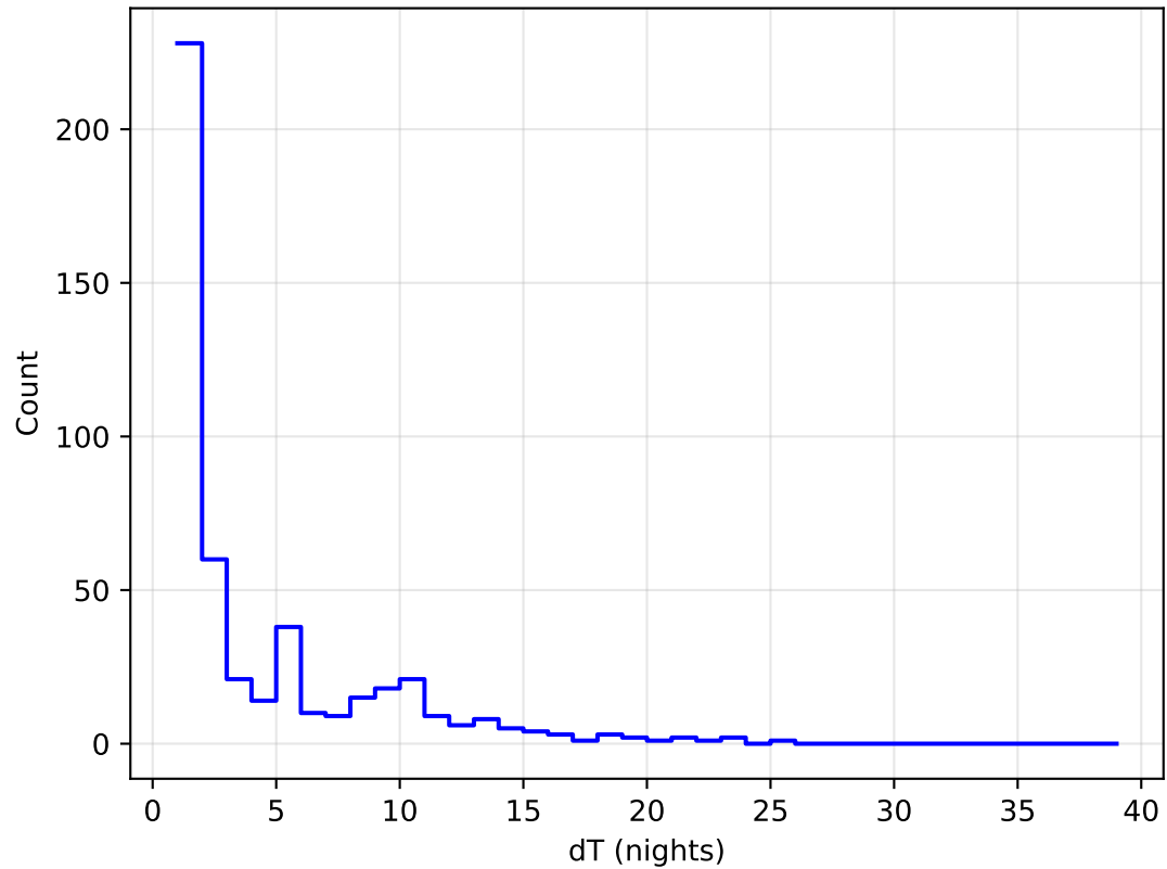
too_elab_r16_d3_ugrizy_v3.4_10yrs all bands: DD: COSMOS Delta Nights Histogram
