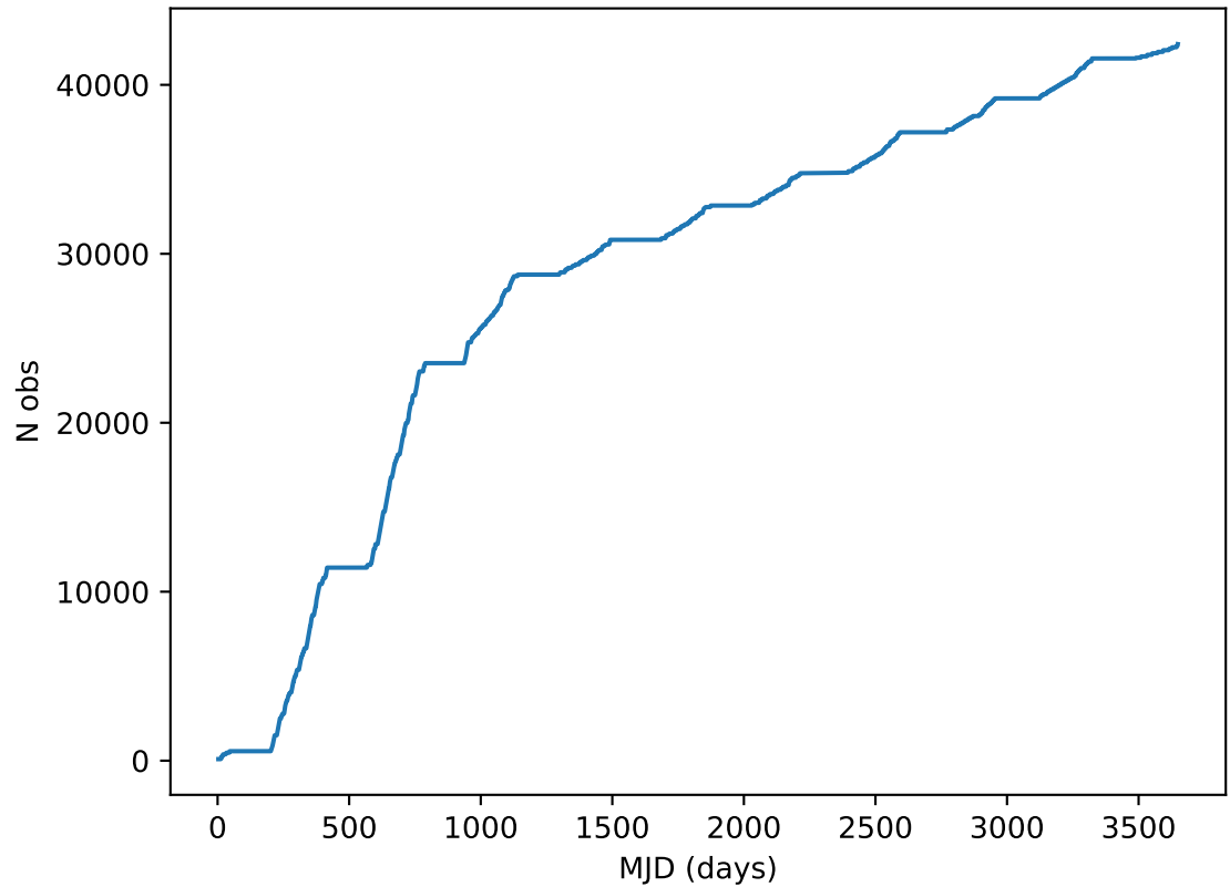
too_elab_r16_d3_ugrizy_v3.4_10yrs all bands: DD: COSMOS Cumulative NVisits
