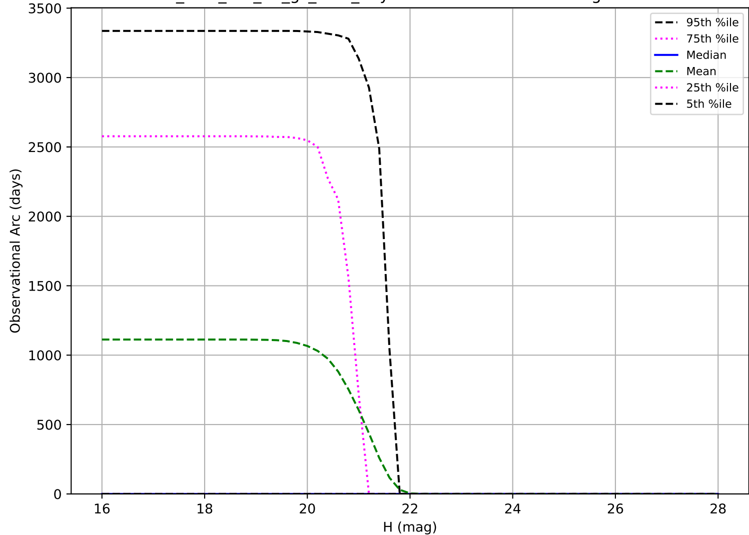
too_elab_r16_d3_gz_v3.4_10yrs: Observational Arc Length Vatra
