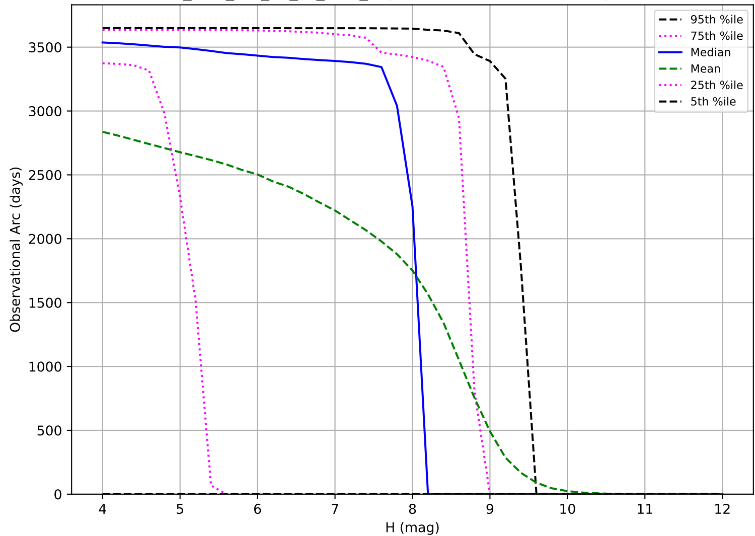
too_elab_r16_d3_gz_v3.4_10yrs: Observational Arc Length TNO
