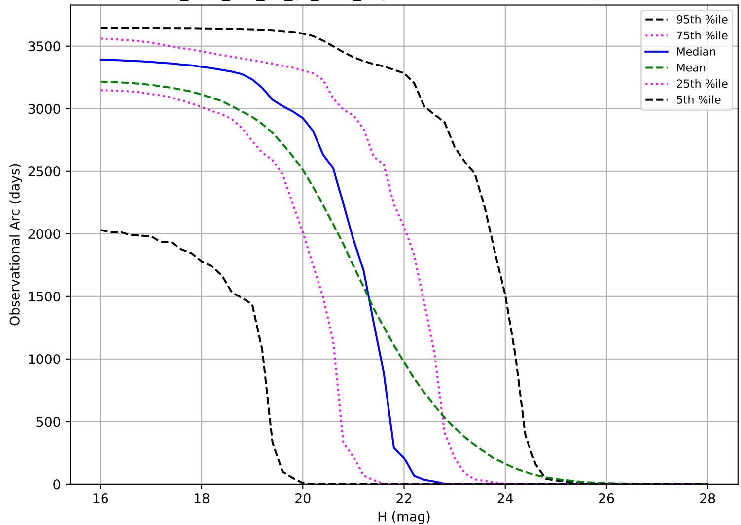
too_elab_r16_d3_gz_v3.4_10yrs: Observational Arc Length PHA
