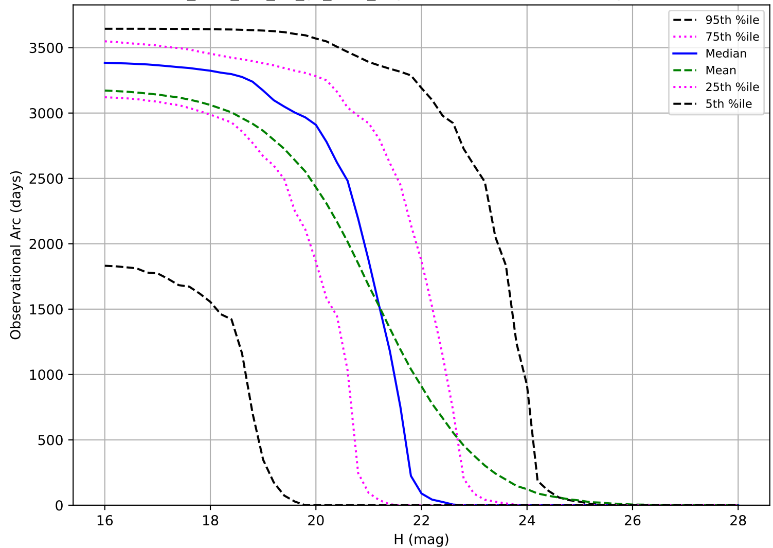
too_elab_r16_d3_gz_v3.4_10yrs: Observational Arc Length NEO
