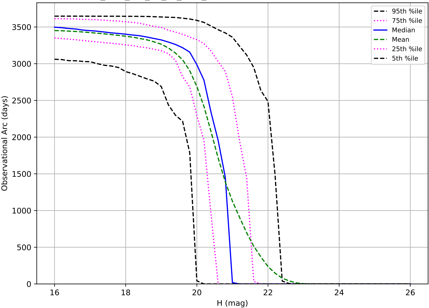
too_elab_r16_d3_gz_v3.4_10yrs: Observational Arc Length MBA
