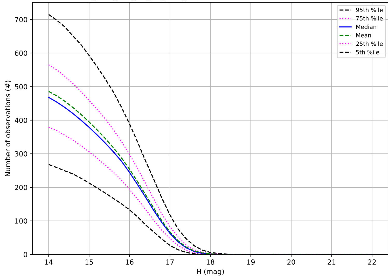
too_elab_r16_d3_gz_v3.4_10yrs: Number of observations Trojan
