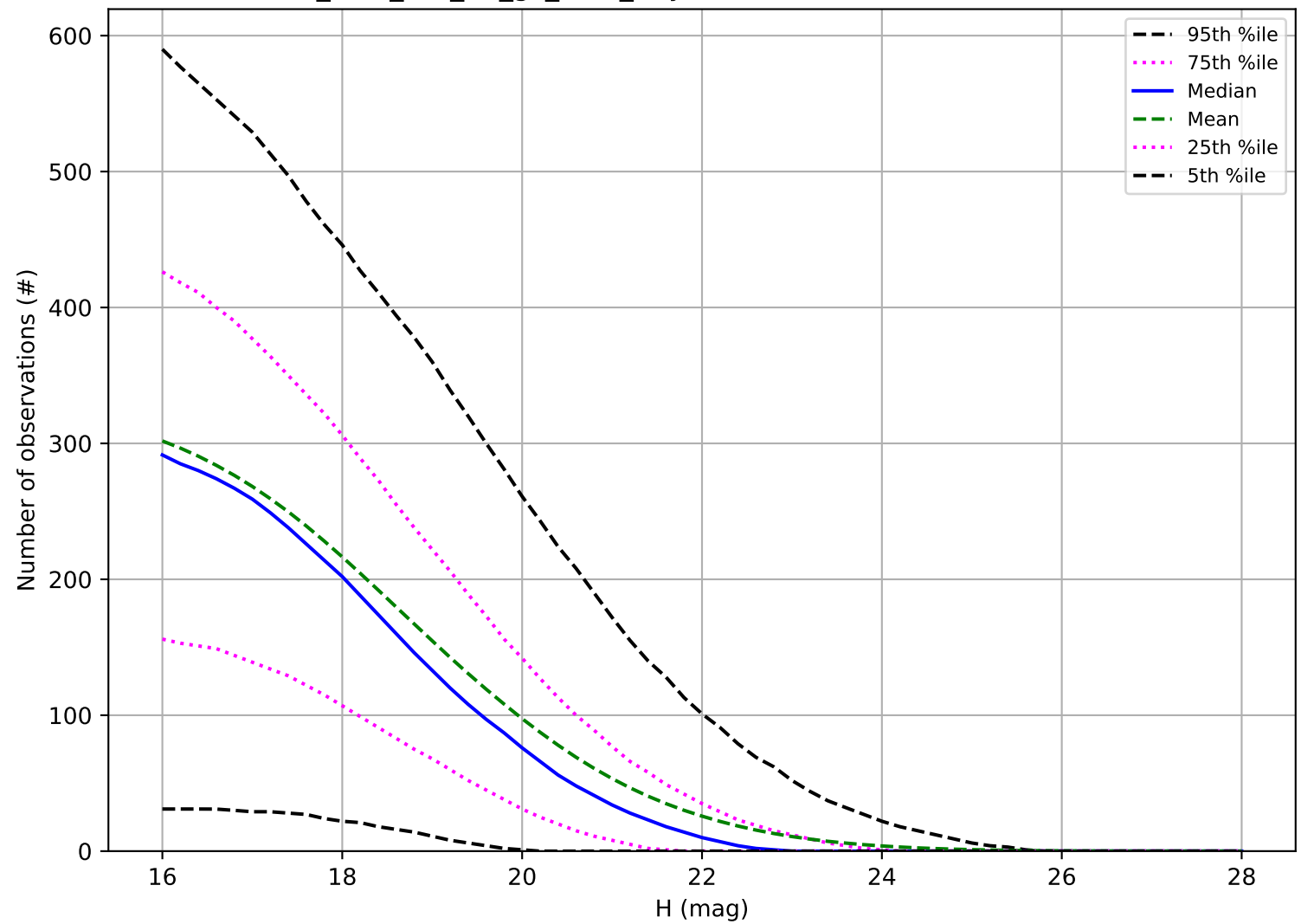
too_elab_r16_d3_gz_v3.4_10yrs: Number of observations NEO
