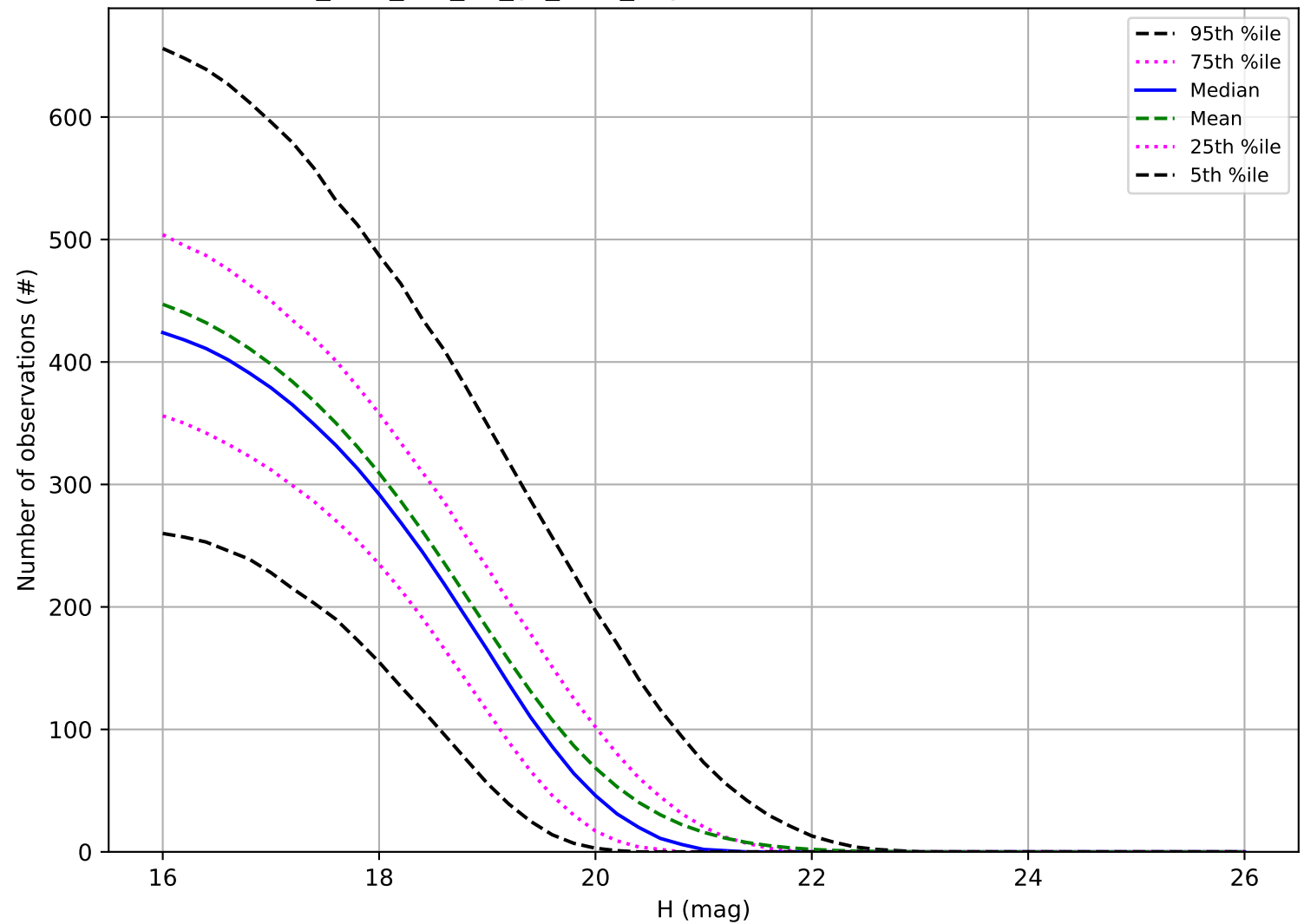
too_elab_r16_d3_gz_v3.4_10yrs: Number of observations MBA
