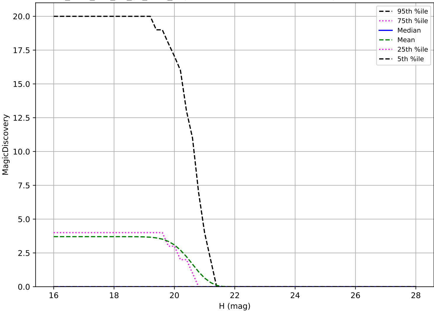
too_elab_r16_d3_gz_v3.4_10yrs: Vatra 6 detections in 60 nights detection loss
