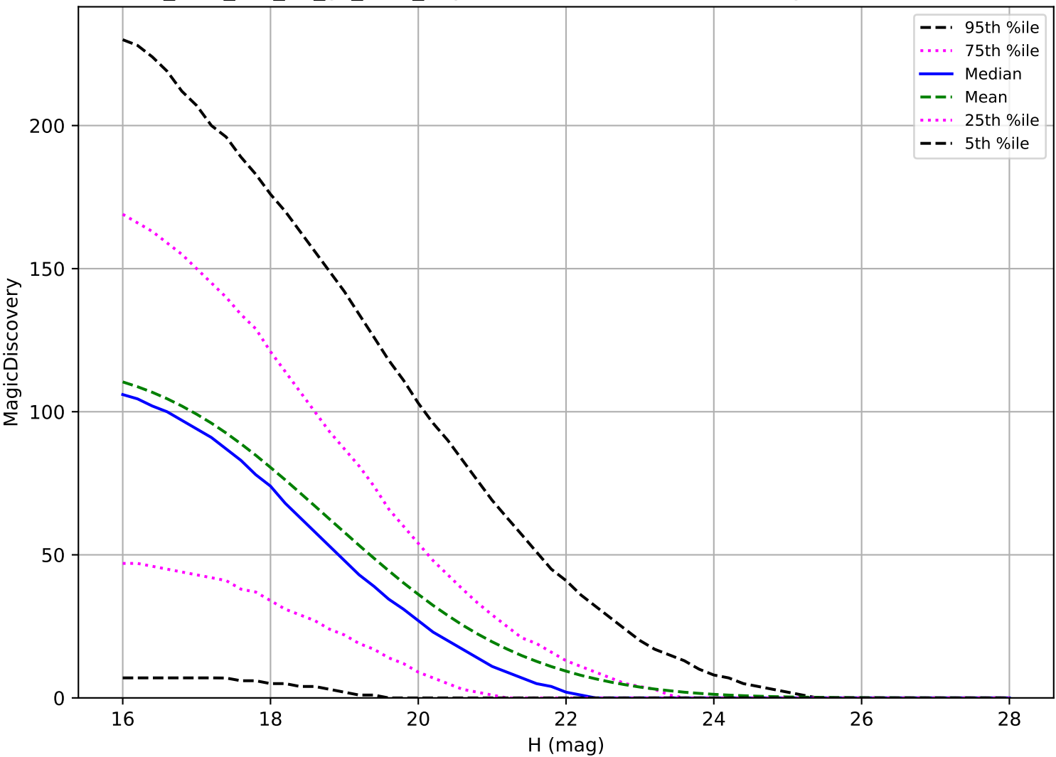
too_elab_r16_d3_gz_v3.4_10yrs: PHA 6 detections in 60 nights detection loss
