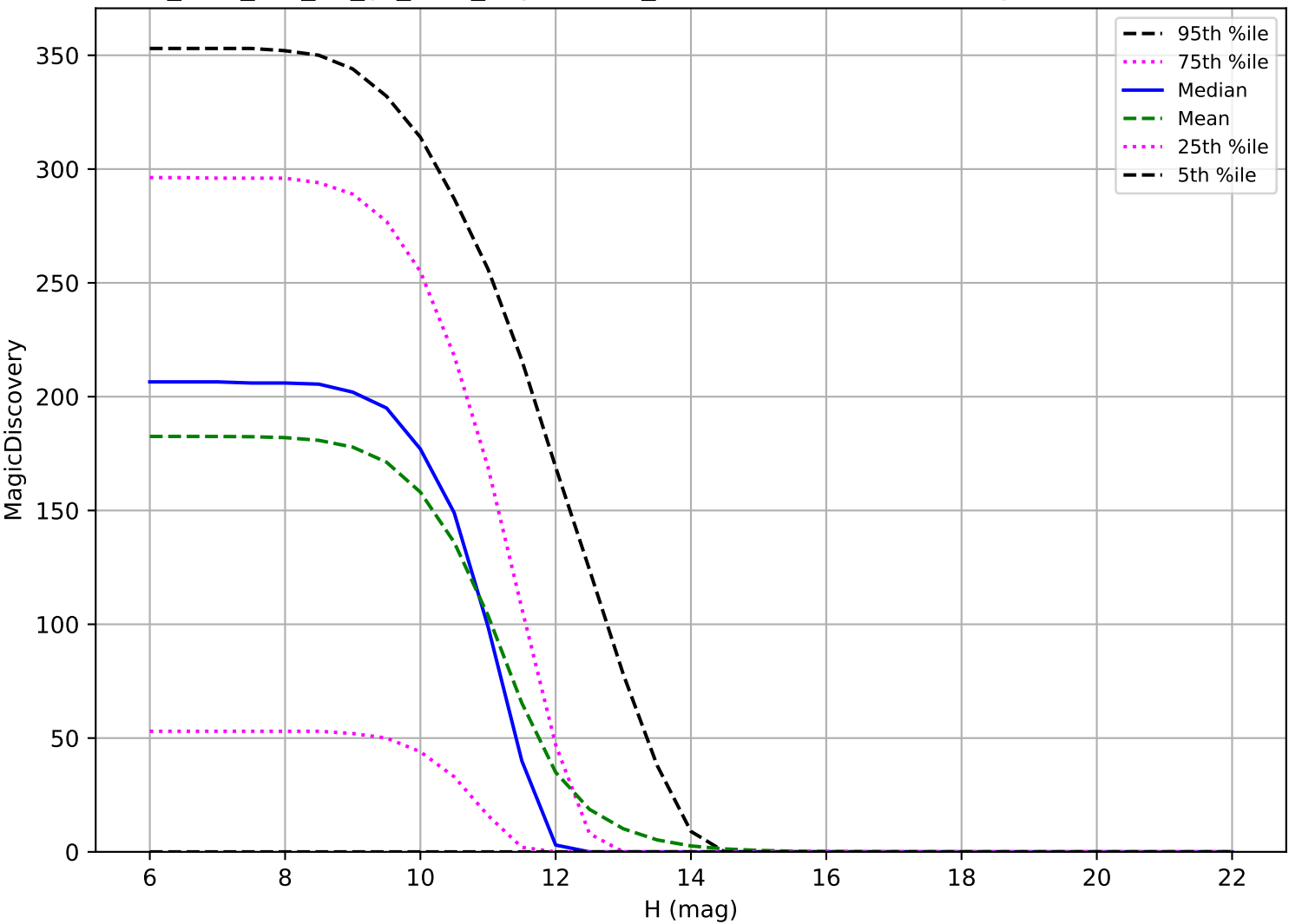
too_elab_r16_d3_gz_v3.4_10yrs: OCC_r20 6 detections in 60 nights detection loss
