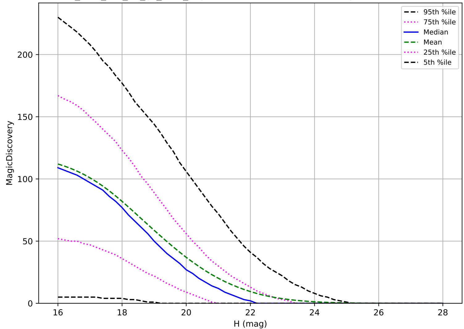
too_elab_r16_d3_gz_v3.4_10yrs: NEO 6 detections in 60 nights detection loss
