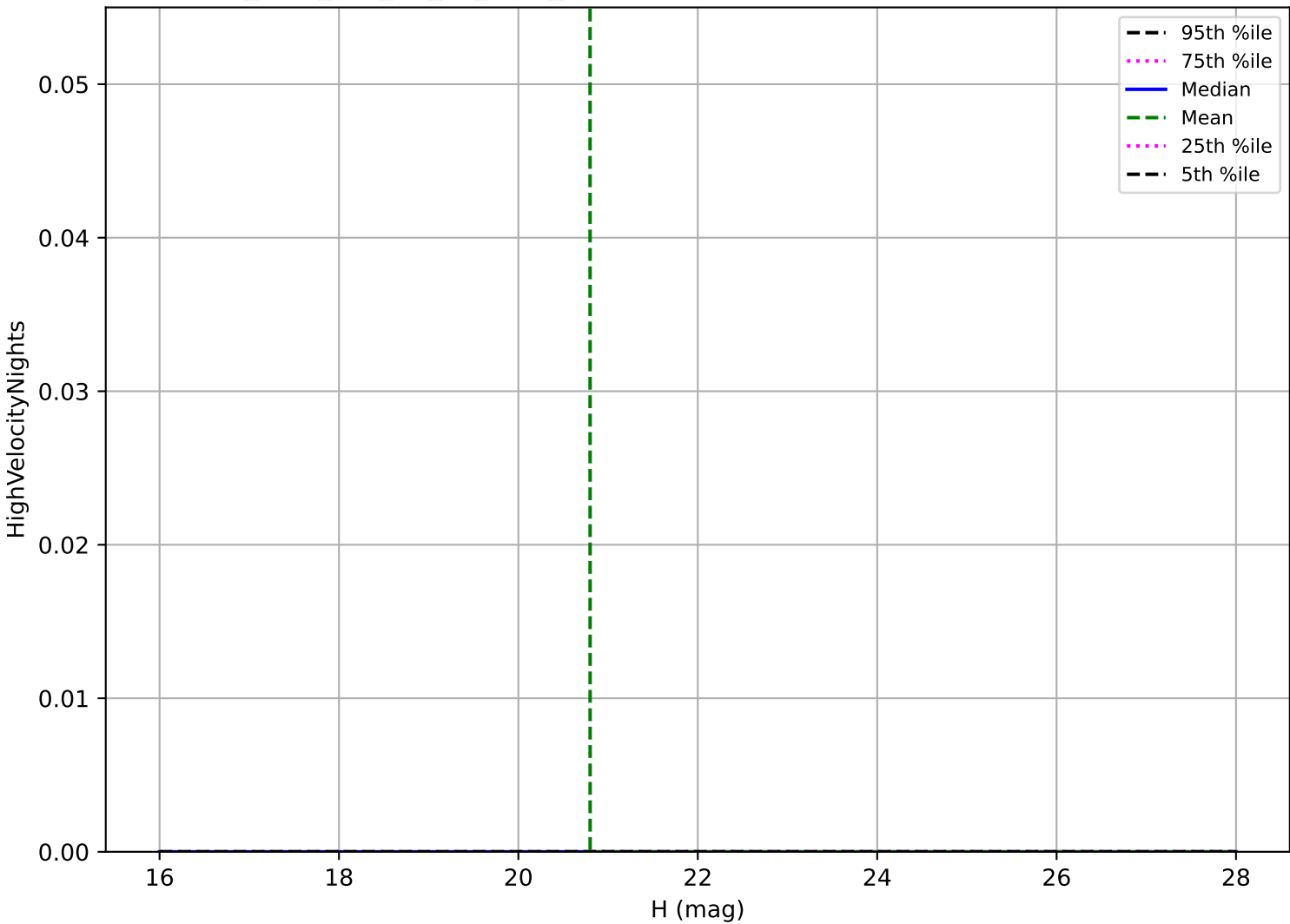
too_elab_r16_d3_gz_v3.4_10yrs: Vatira High velocity pair detection loss
