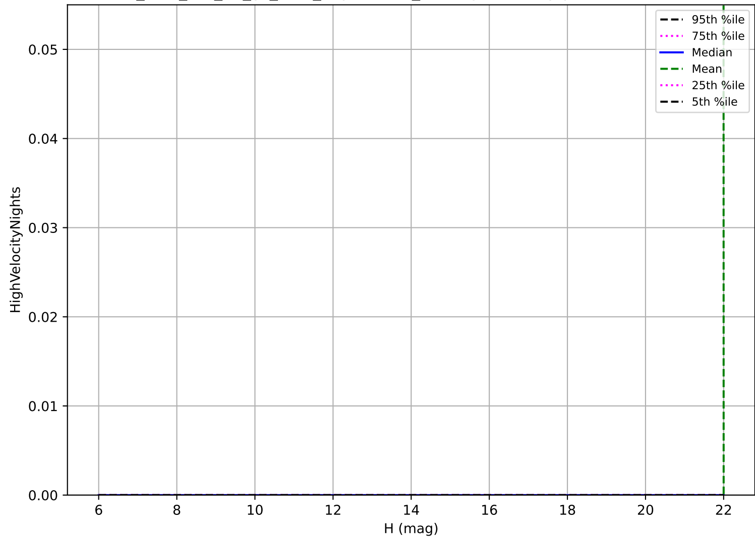
too_elab_r16_d3_gz_v3.4_10yrs: OCC_r20 High velocity pair detection loss
