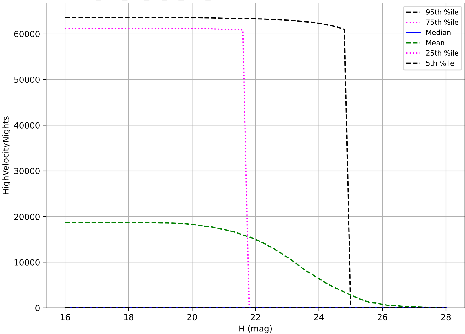
too_elab_r16_d3_gz_v3.4_10yrs: NEO High velocity pair detection loss
