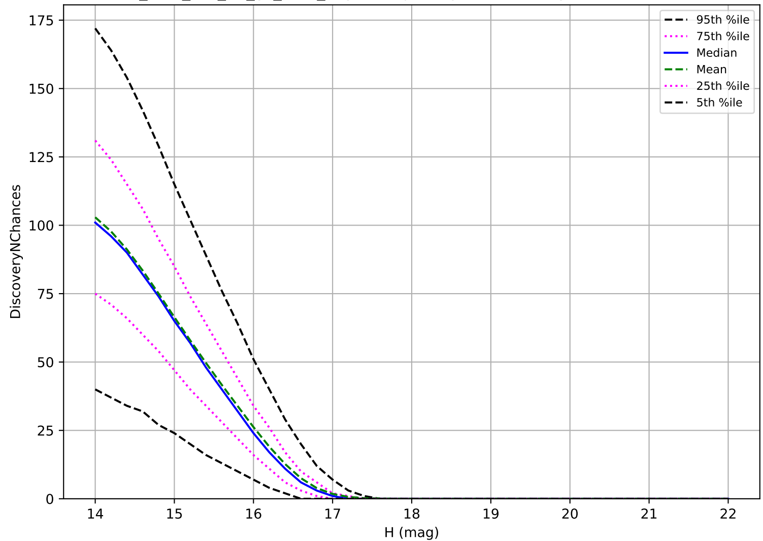
too_elab_r16_d3_gz_v3.4_10yrs: Trojan 3 pairs in 15 nights detection loss
