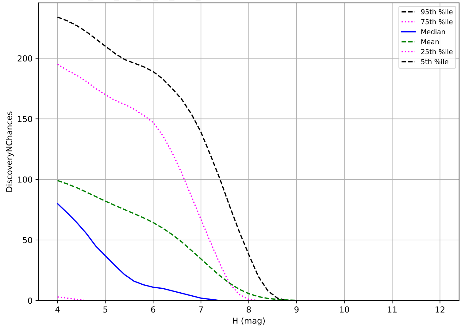
too_elab_r16_d3_gz_v3.4_10yrs: TNO 3 pairs in 15 nights detection loss
