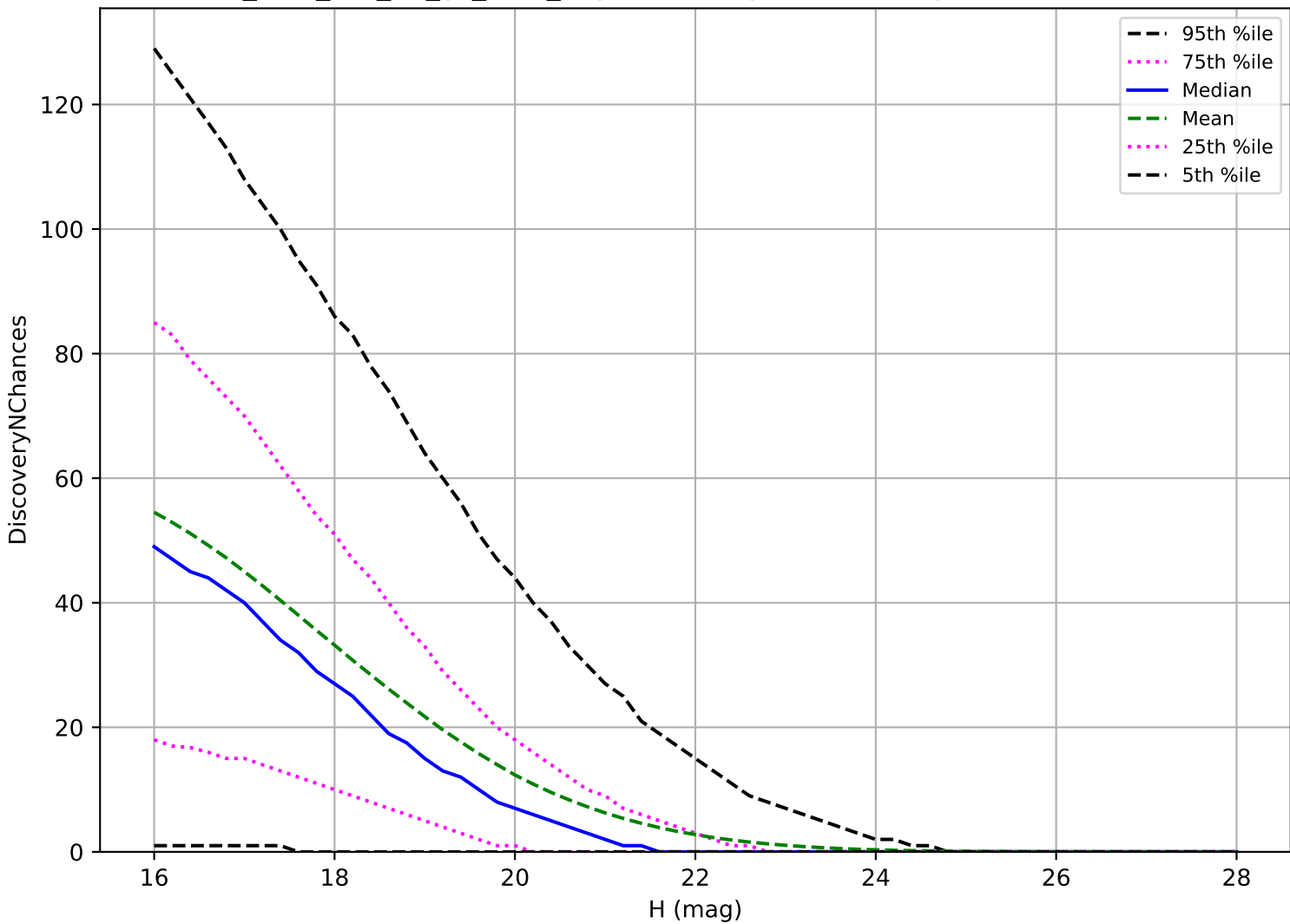
too_elab_r16_d3_gz_v3.4_10yrs: PHA 3 pairs in 15 nights detection loss
