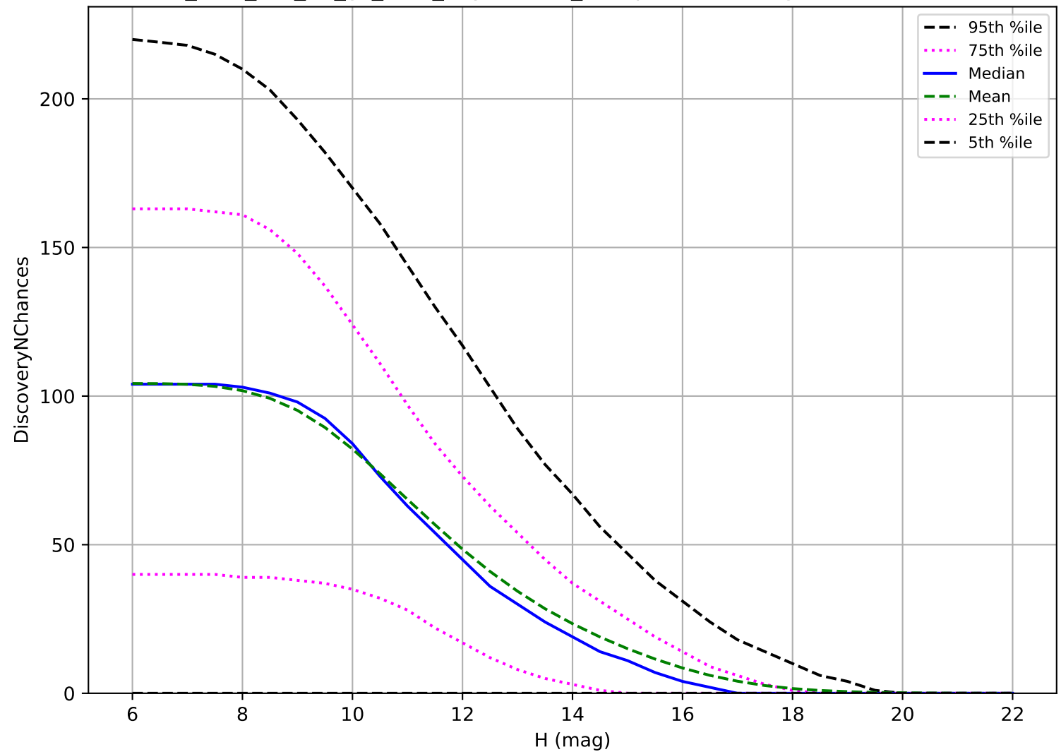
too_elab_r16_d3_gz_v3.4_10yrs: OCC_r5 3 pairs in 15 nights detection loss
