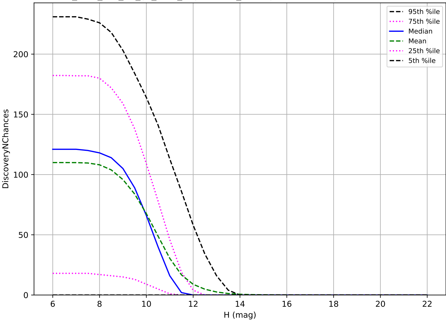
too_elab_r16_d3_gz_v3.4_10yrs: OCC_r20 3 pairs in 15 nights detection loss
