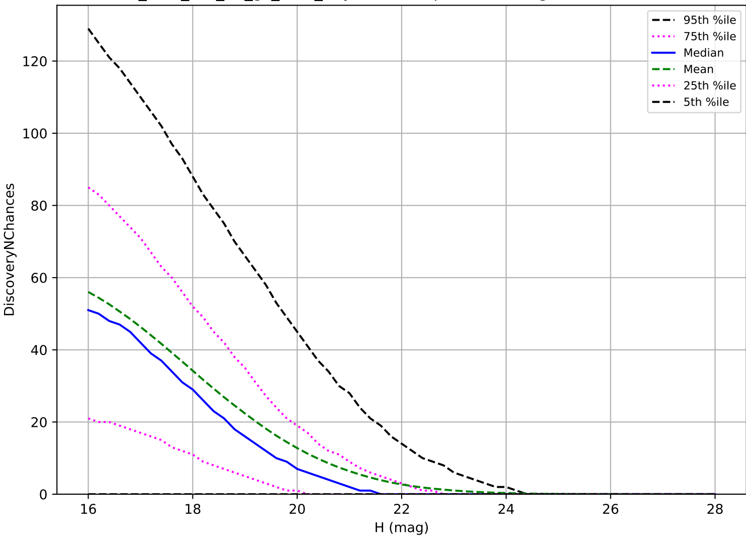
too_elab_r16_d3_gz_v3.4_10yrs: NEO 3 pairs in 15 nights detection loss
