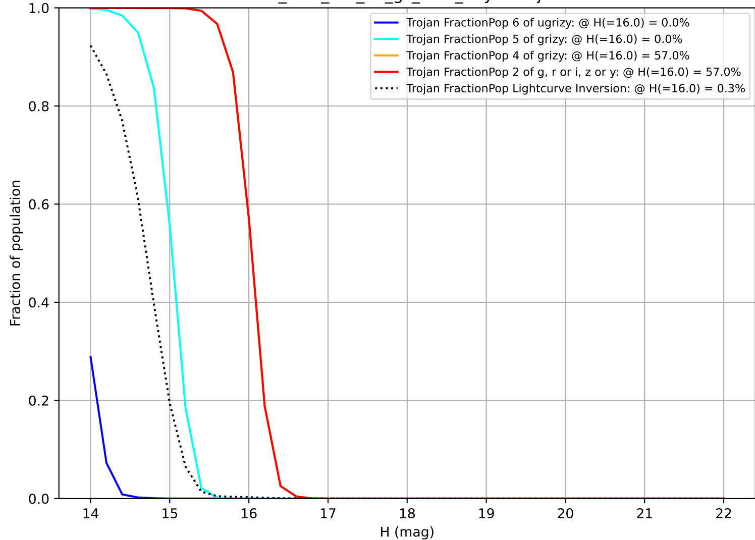
too_elab_r16_d3_gz_v3.4_10yrs Trojan
