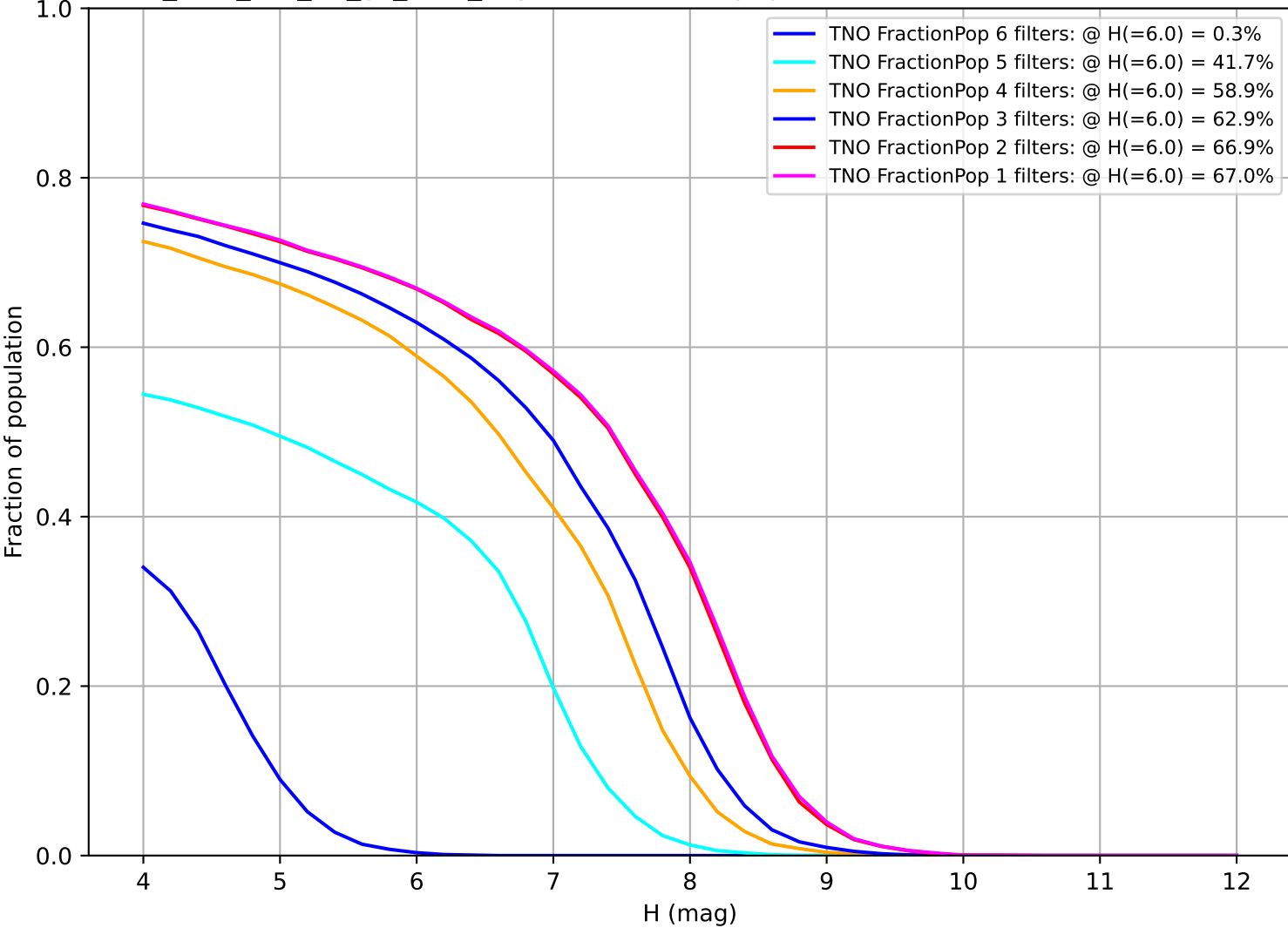
too_elab_r16_d3_gz_v3.4_10yrs: Fraction of population with colors in X filters TNO
